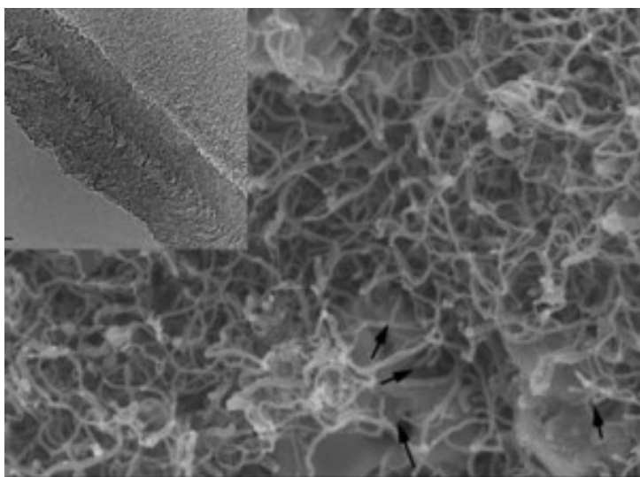
SEM - Carbon Nanotube Nickel
