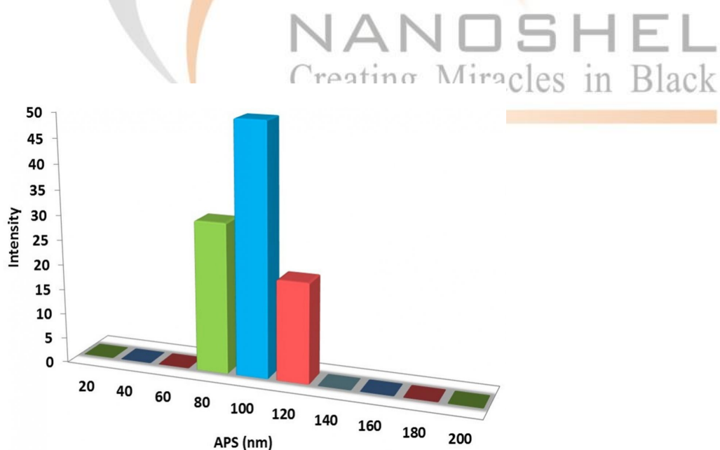
Particles Size Analysis - Lithium Titanate Nanoparticles
