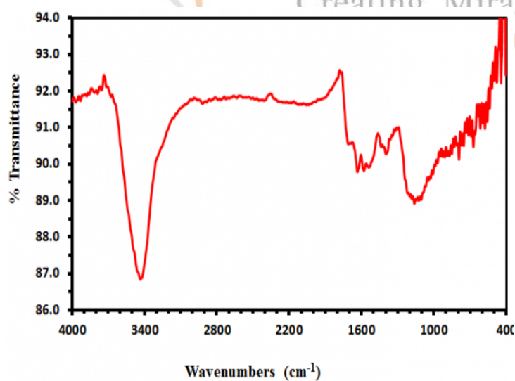
FTIR Spectra of Few Walled Carbon Nanotubes
