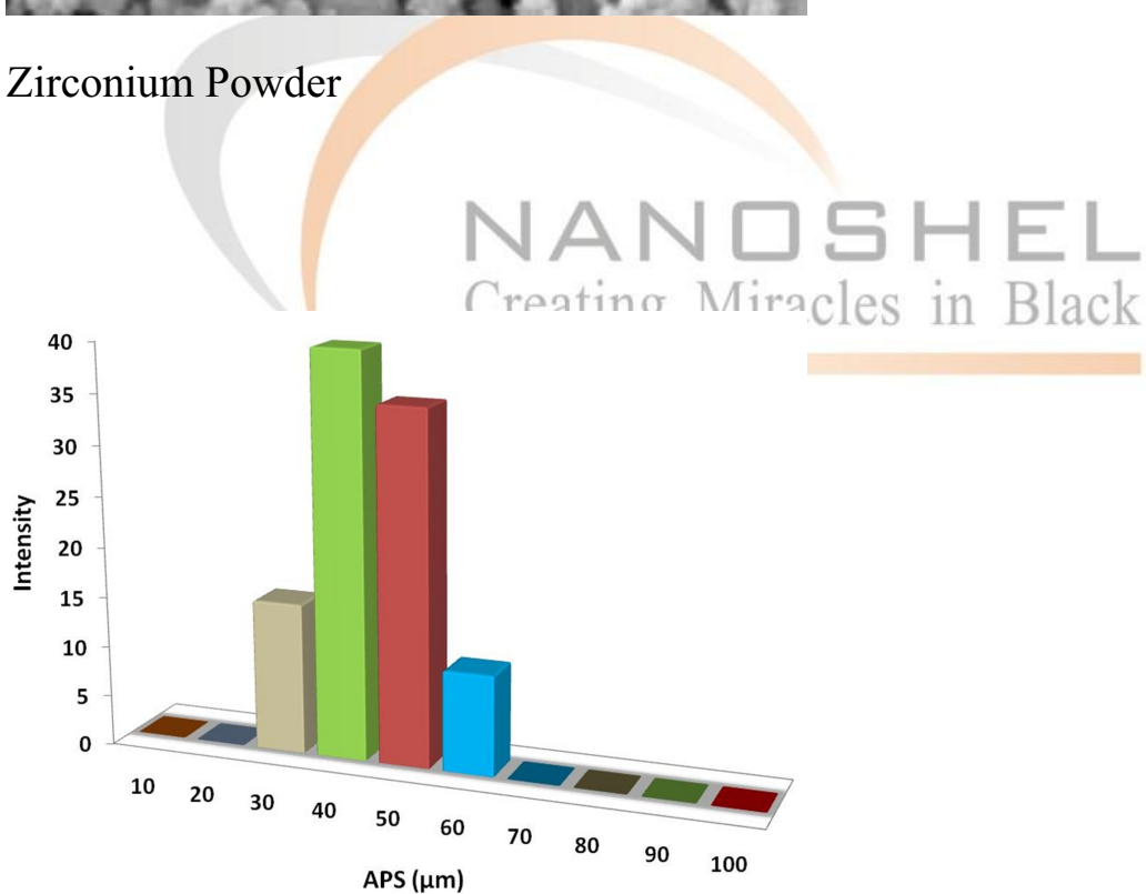
Particles Size Analysis – Zr Powder
