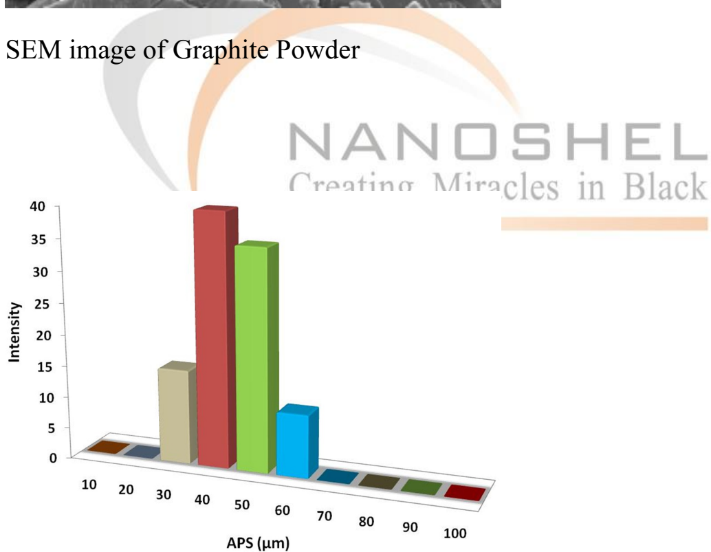
Particles Size Analysis - Graphite Powder
