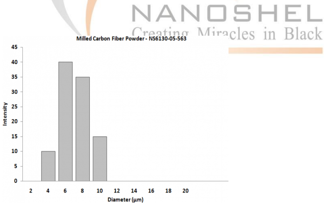
Milled Carbon Fiber – Size Analysis
