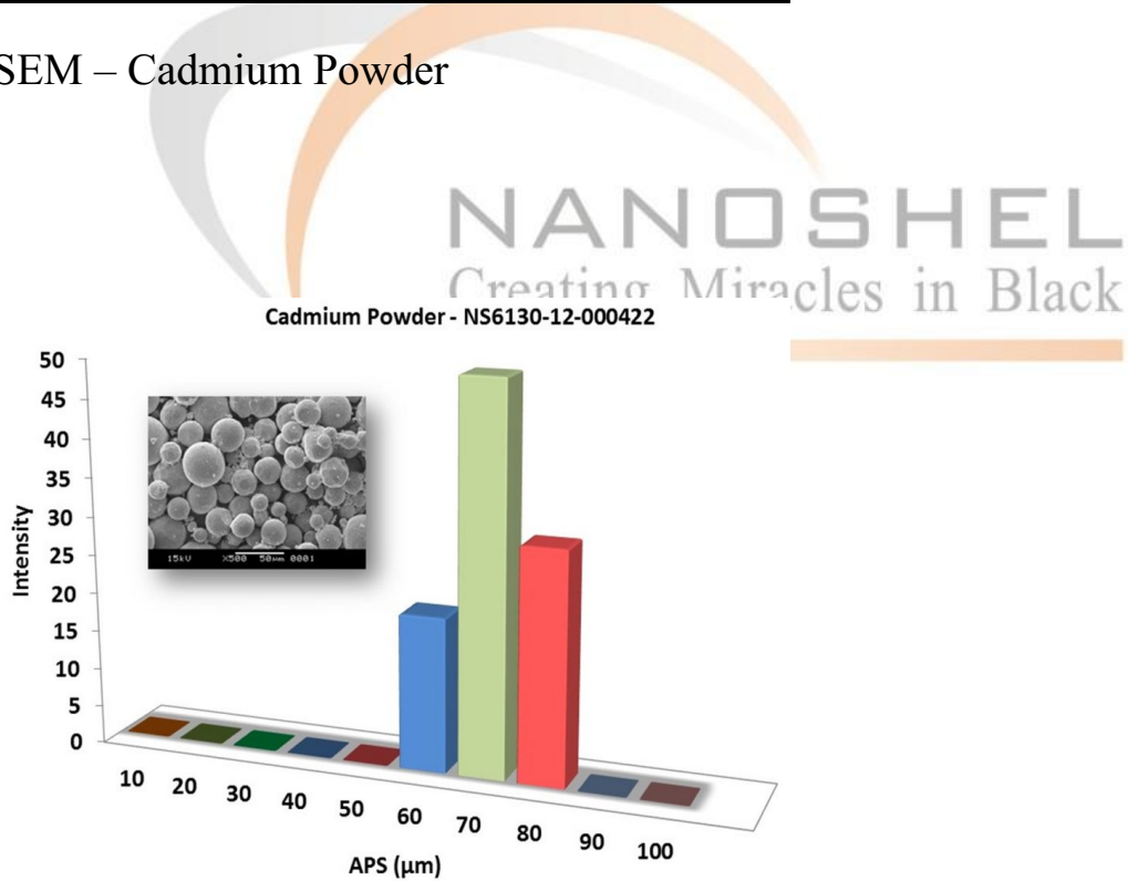
Particles Size Analysis – Cd Powder
