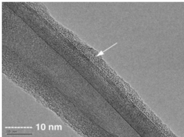
TEM of CNT Multiwall
