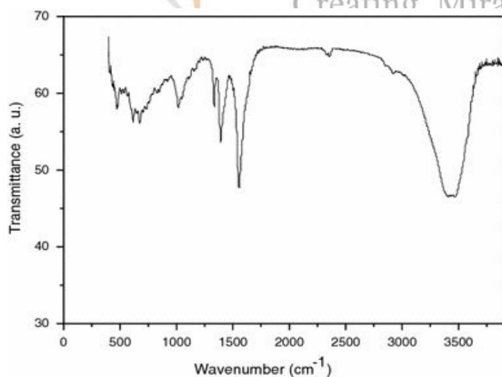
FTIR Spectra of Zinc Acetate Nanoparticles
