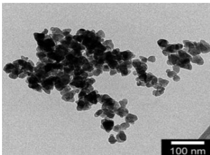
Zinc Acetate Nanoparticles SEM/TEM
