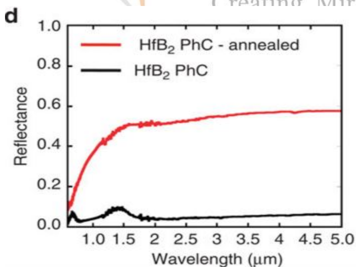
Reflectance spectra of Hafnium Boride
