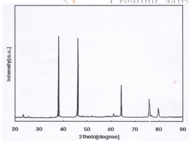
X-Ray Graph of Vanadium Carbide
