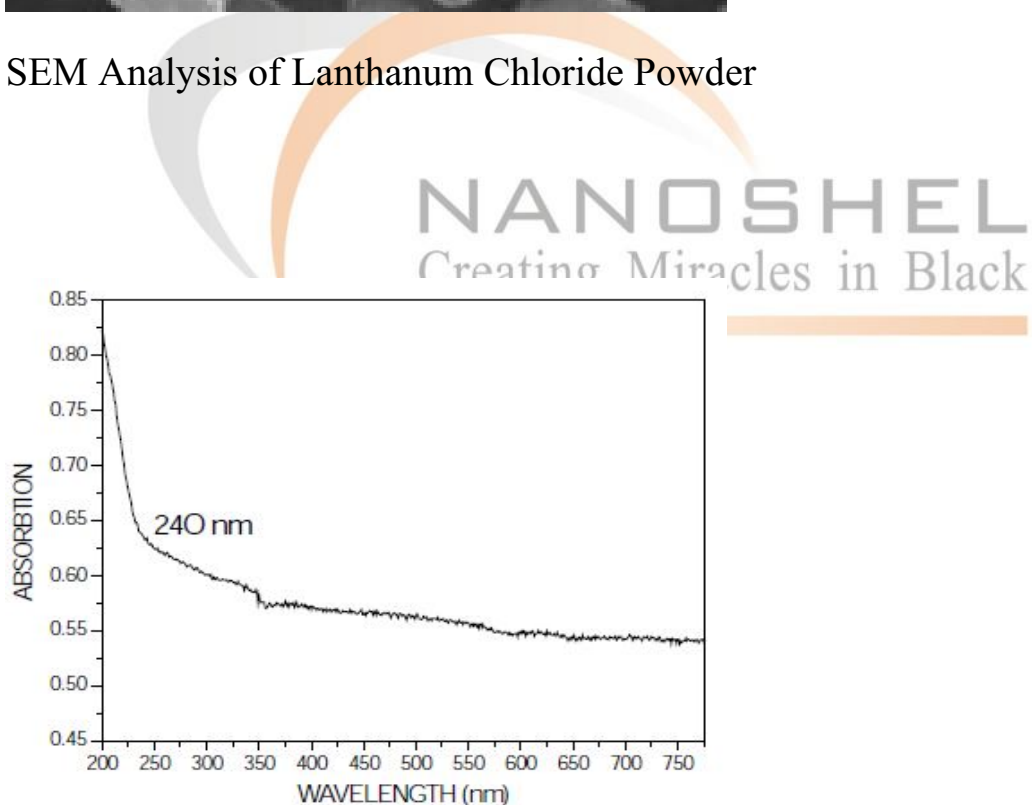
UV/Vis Spectra of Lanthanum Chloride Powder
