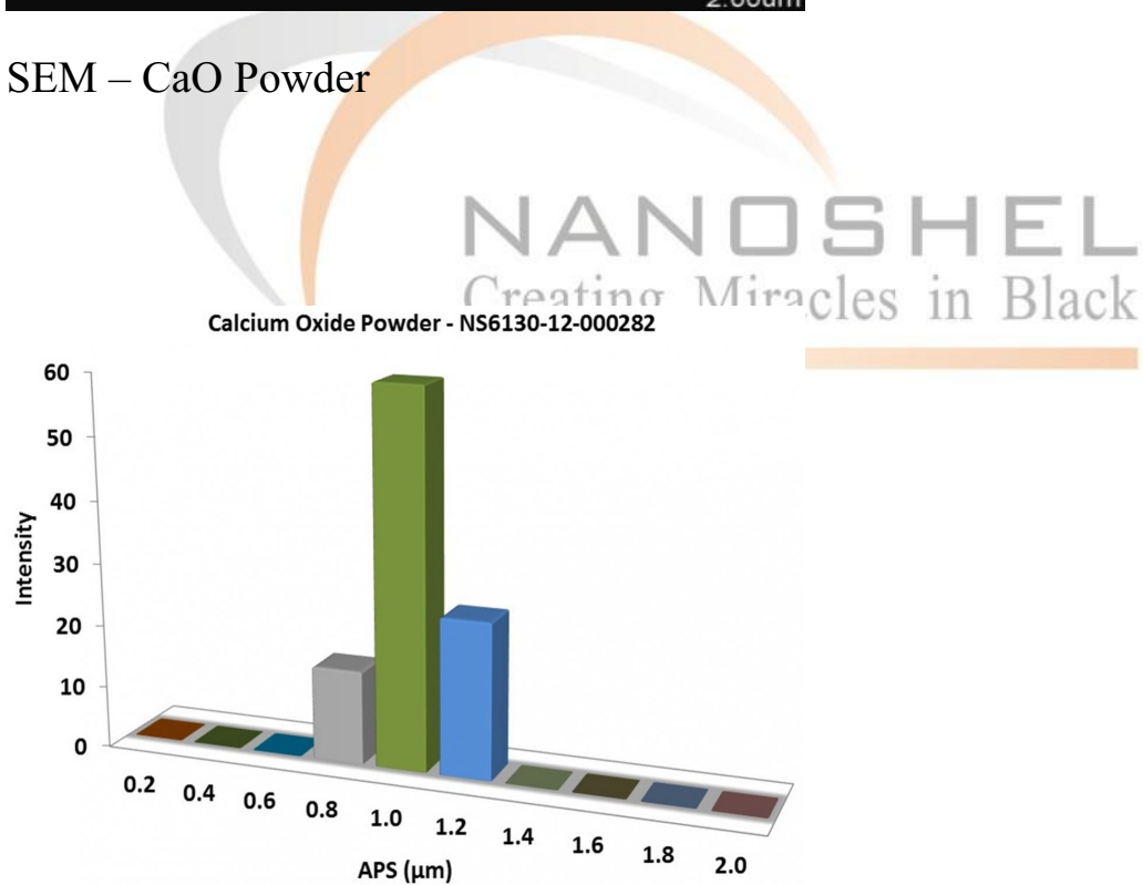
Particles Size Analysis – Calcium Oxide Powder
