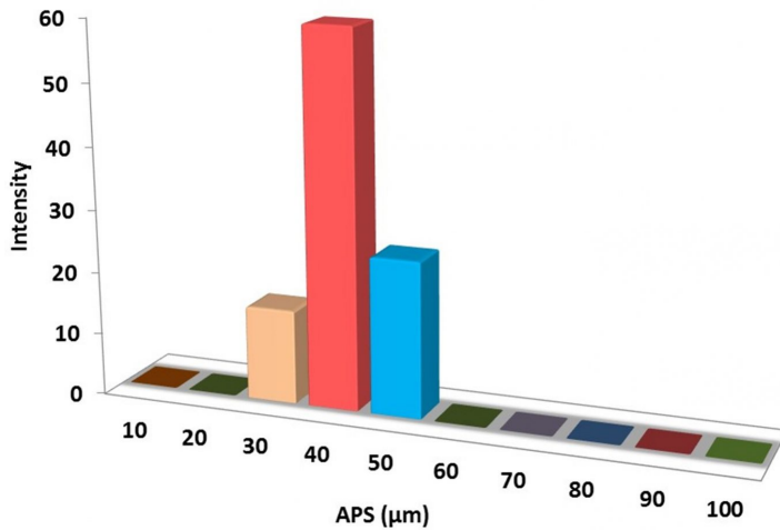
Particles Size Analysis – Germanium Oxide Powder
