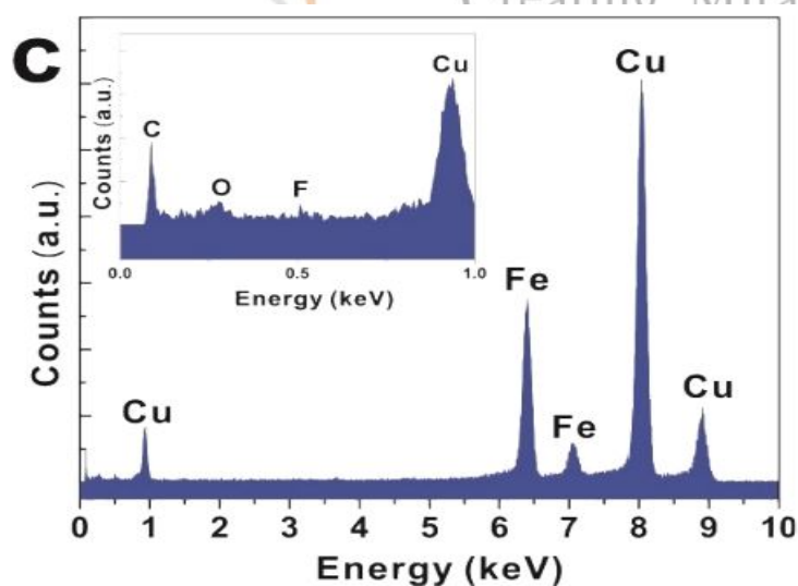
Iron Fluoride Micropowder EDX Spectra
