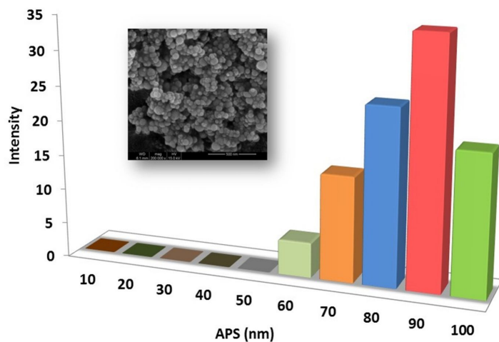
Particles Size Analysis – Titanium Silicate
