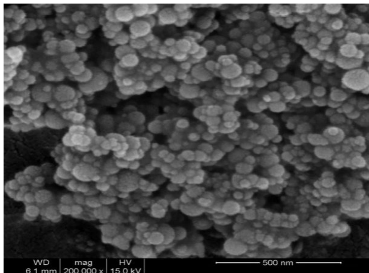
SEM – TiSiO 4 Nanoparticles
