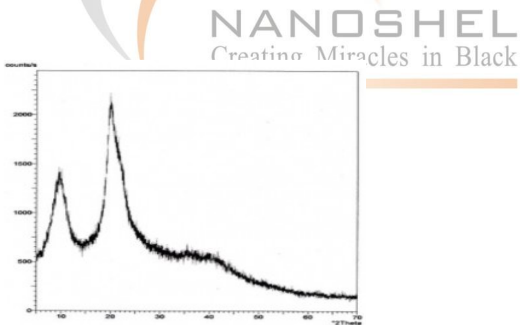
XRD diffractogram High Density Chitosan
