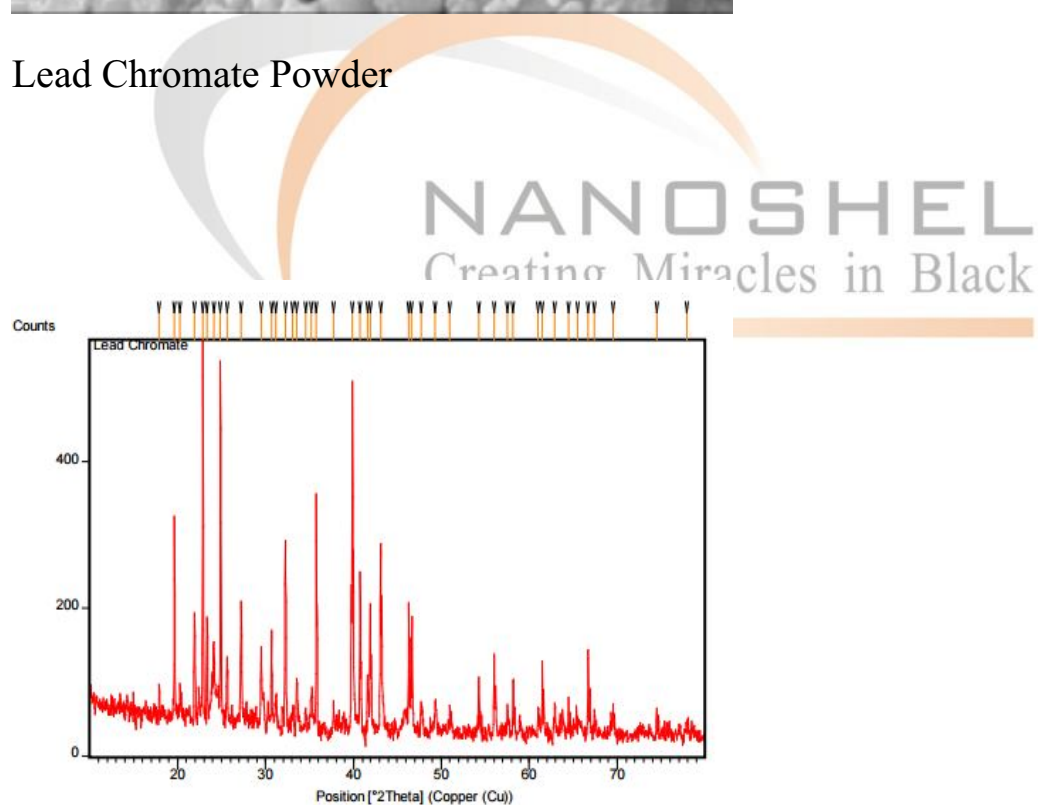
XRD - Lead Chromate Powder
