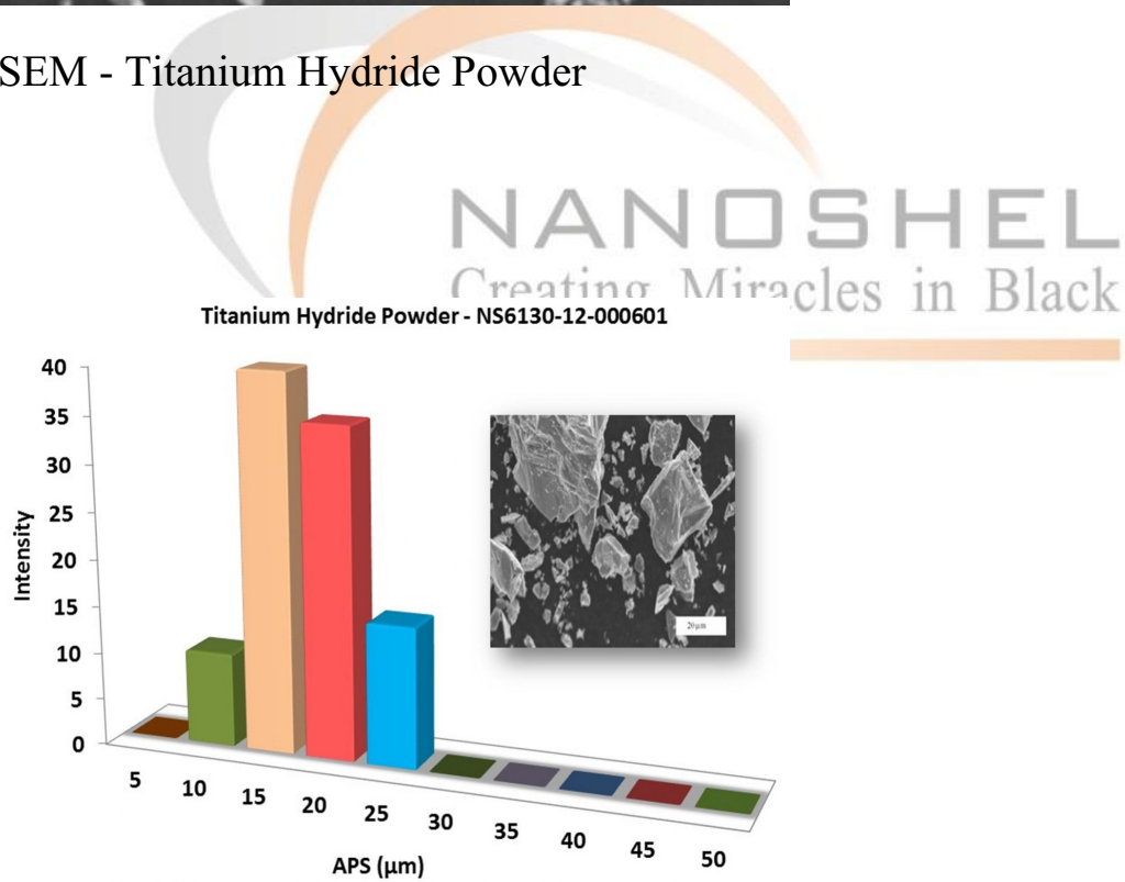
Particles Size Analysis - TiH 2 Powder
