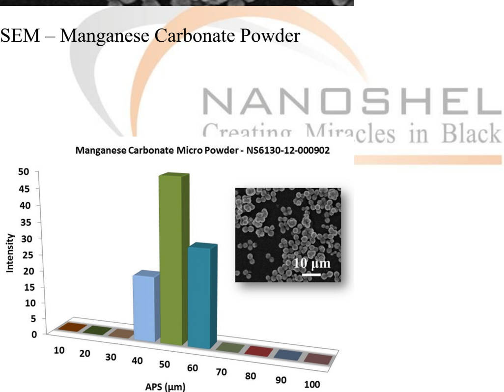
Particles Size Analysis – MnCO 3 Powder
