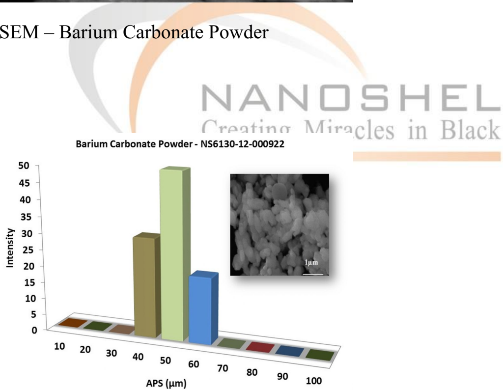
Particles Size Analysis – BaCO 3 Powder
