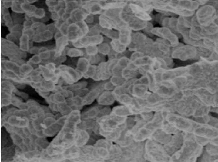
SEM – Gallium Nitride Powder
