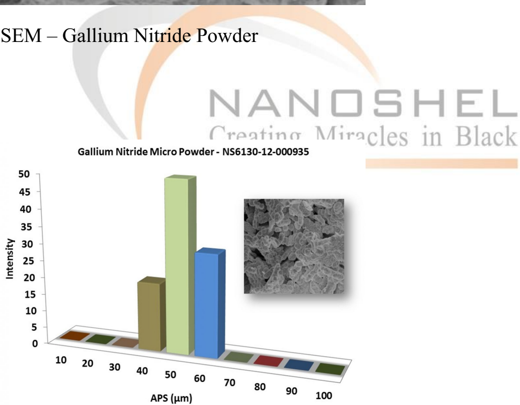
Particles Size Analysis – GaN Powder
