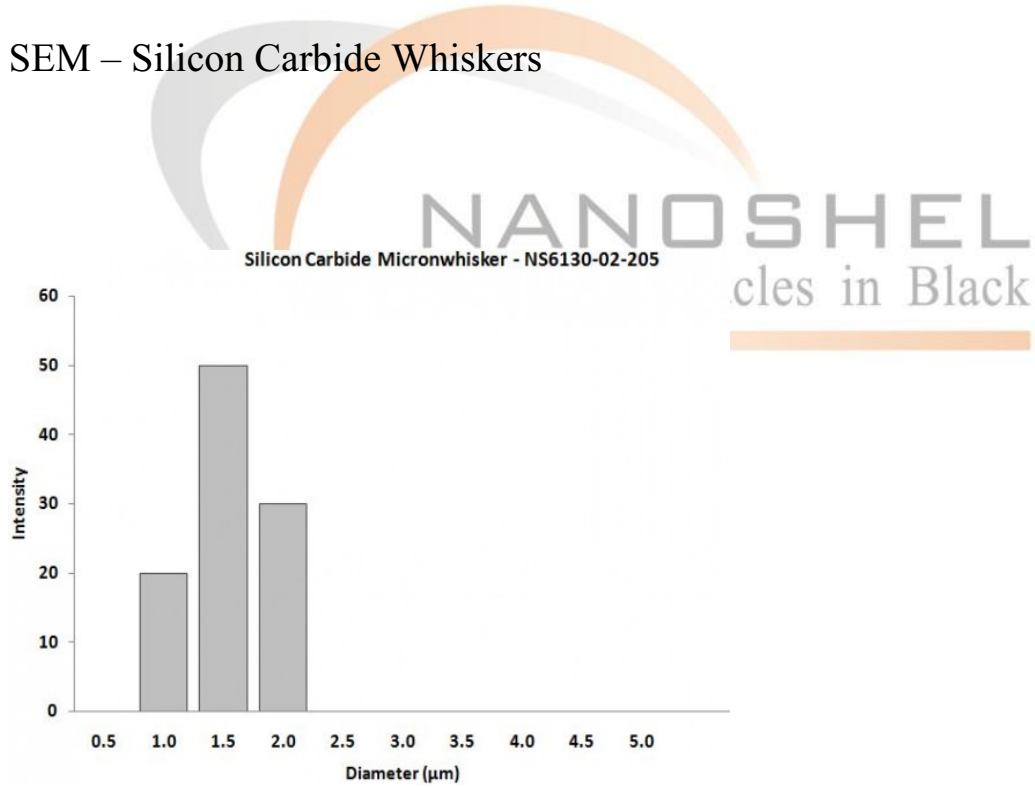
Silicon Carbide Whiskers – Size Analysis
