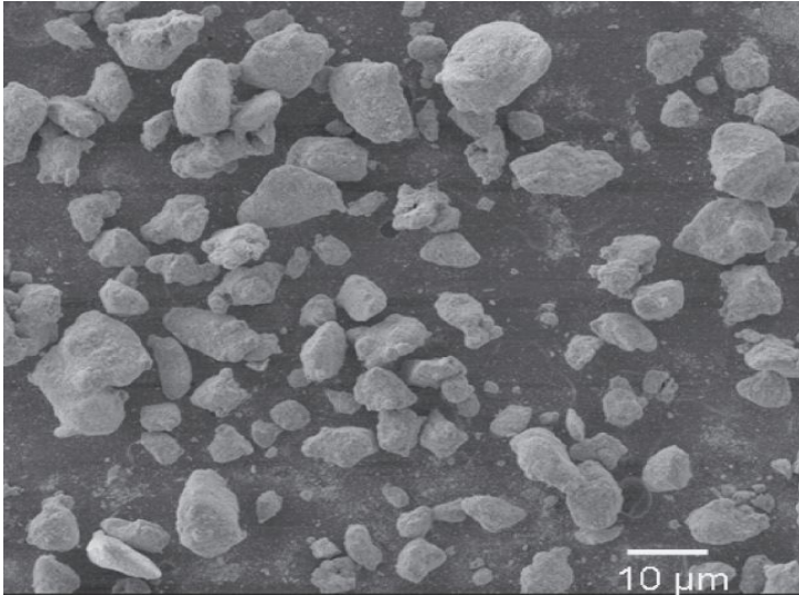
SEM – ZrC Micro Powder
