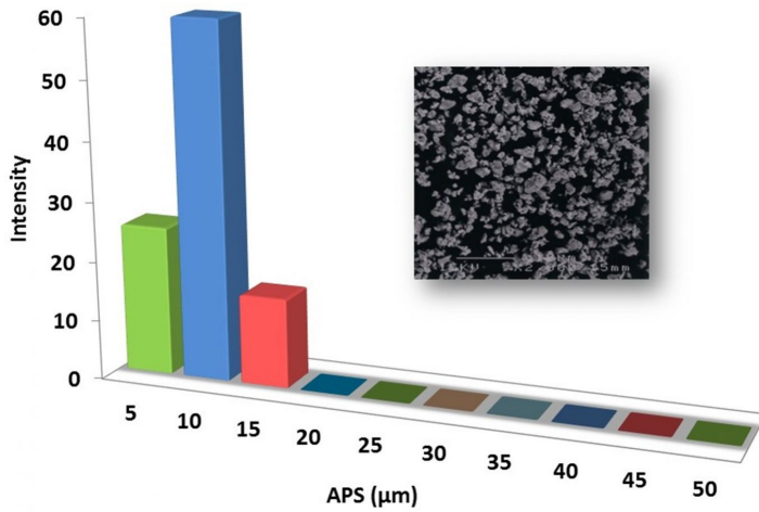
Particles Size Analysis – TaB2 Powder
