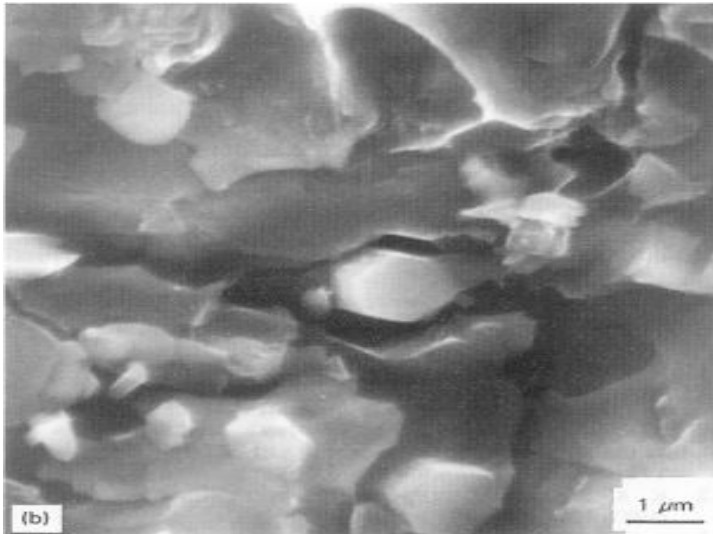
SEM – Silicon Carbide Fine Powder
