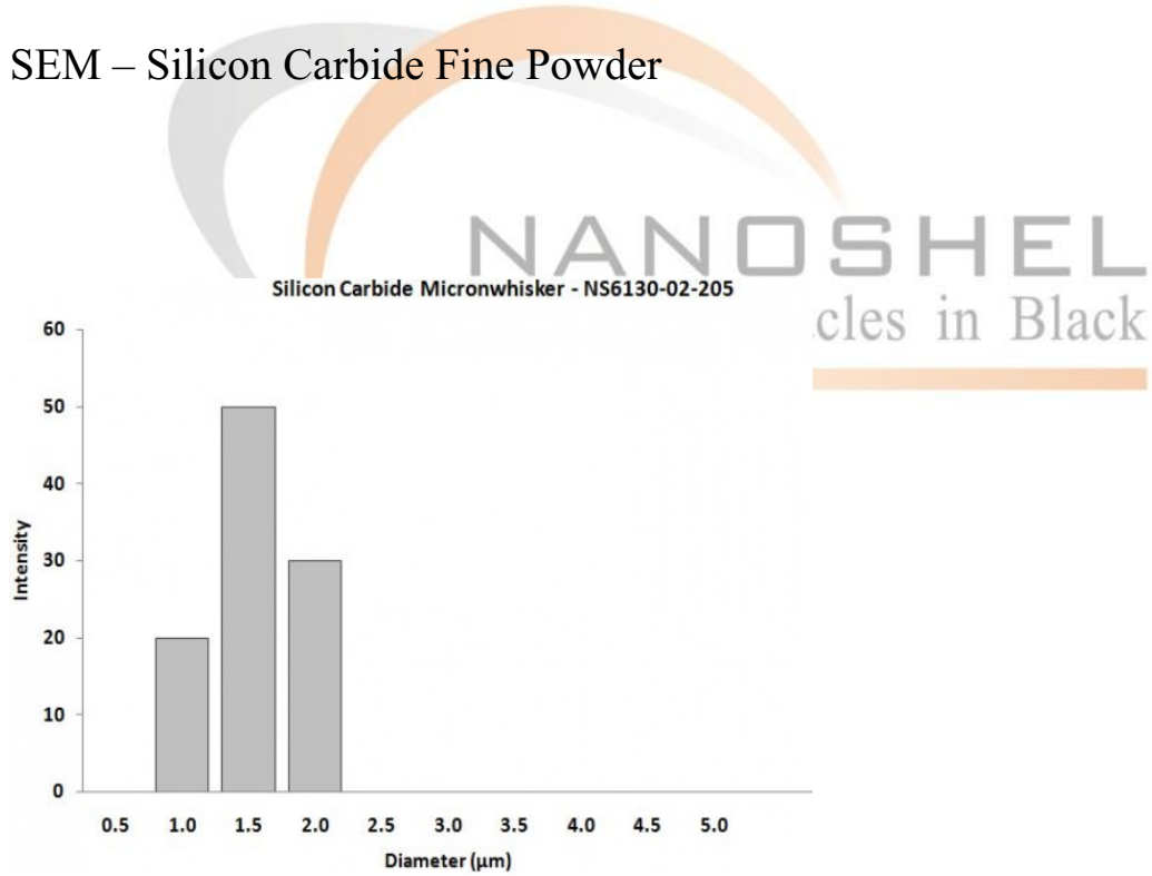
Silicon Carbide – Size Analysis
