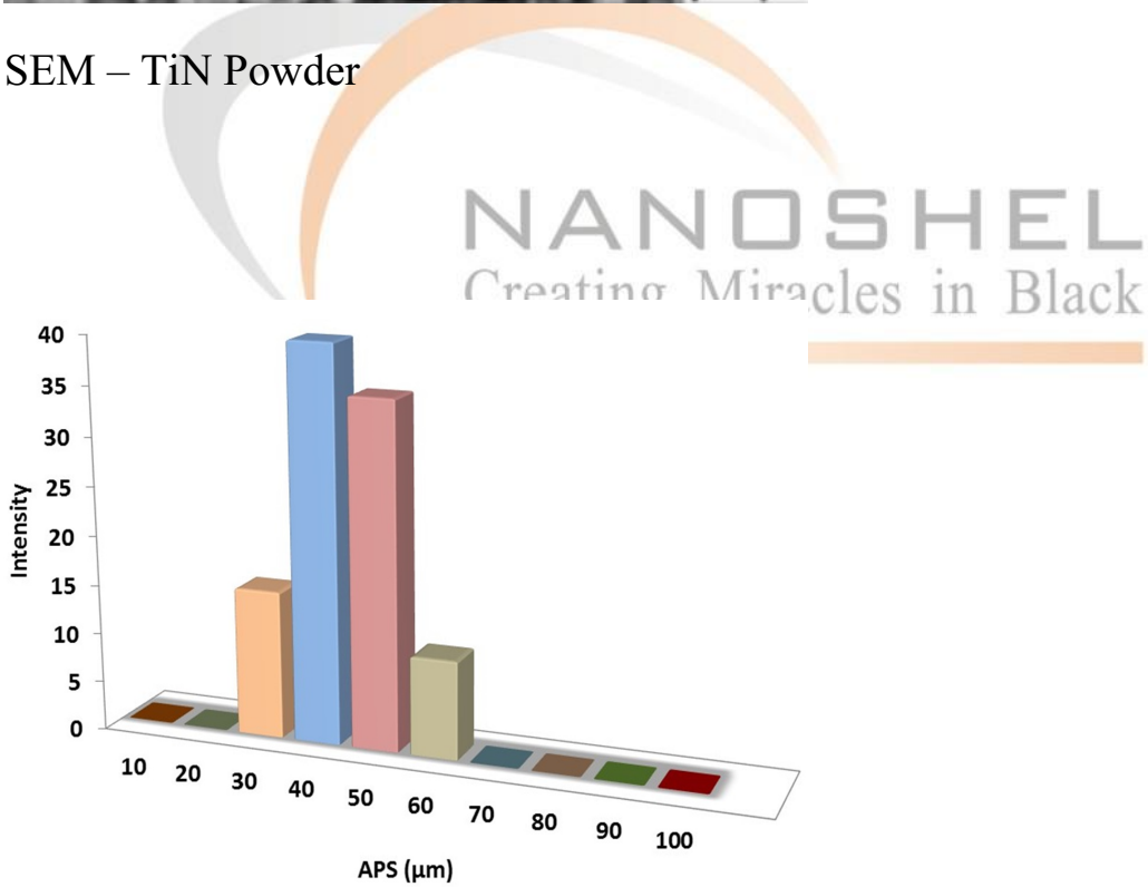
Particles Size Analysis – TiN Powder
