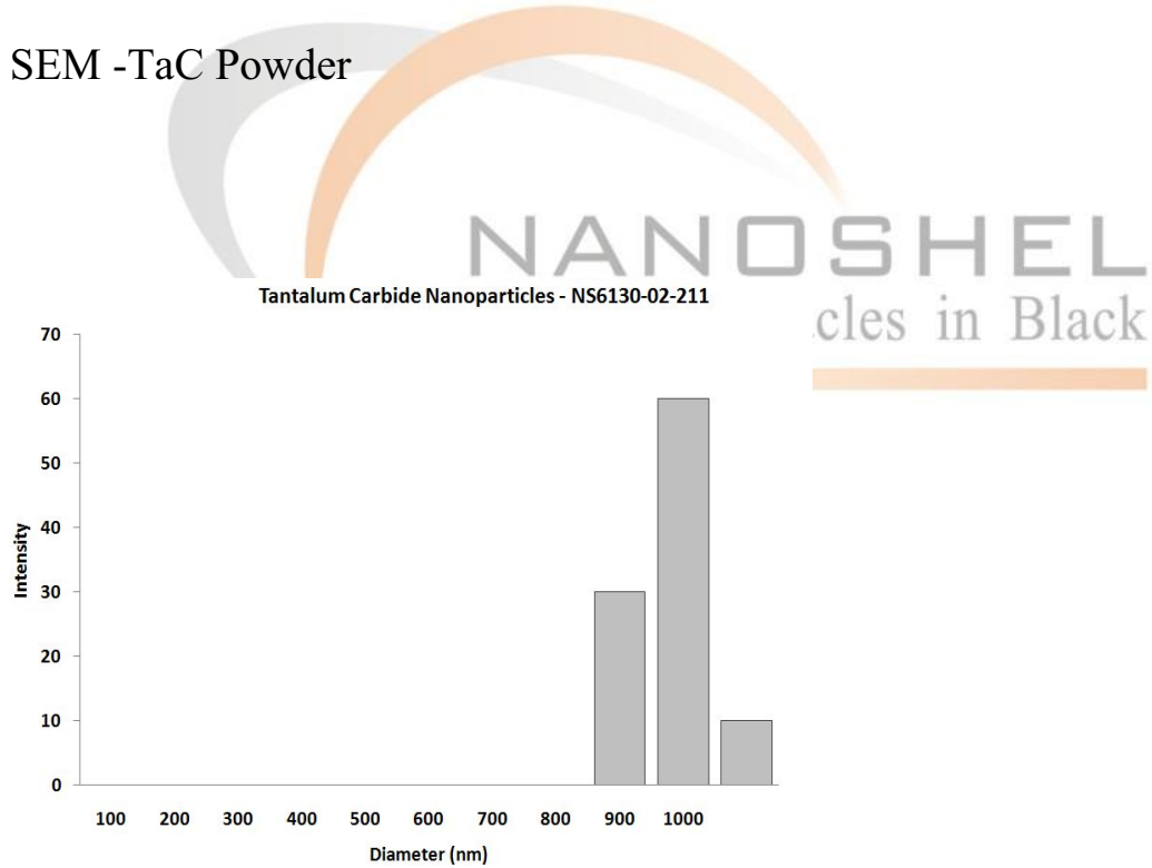
TaC Nanoparticles – Size Analysis
