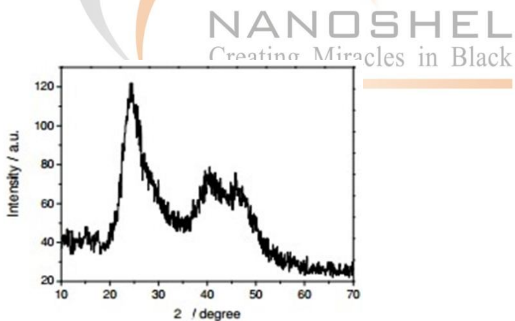
XRD pattern of CdTe QD
