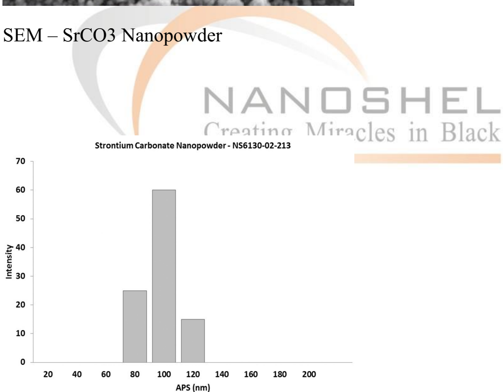
Size Analysis – Strontium Carbonate Nanoparticles
