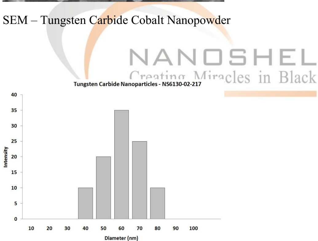
Tungsten Carbide Nanoparticles – Size Analysis
