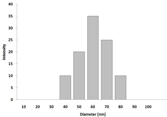
Tungsten Carbide Nanoparticles – Size Analysis
