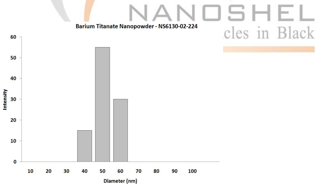
Barium Titanate Nanoparticles – Size Analysis
