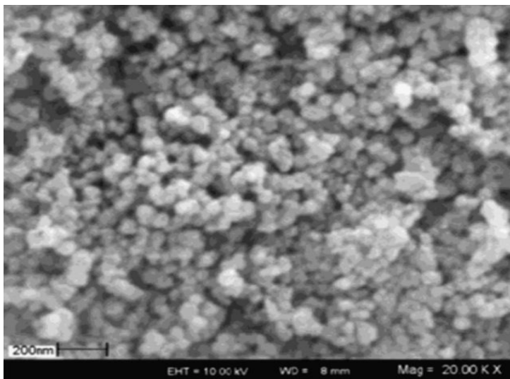
SEM - Calcium Hydroxide
