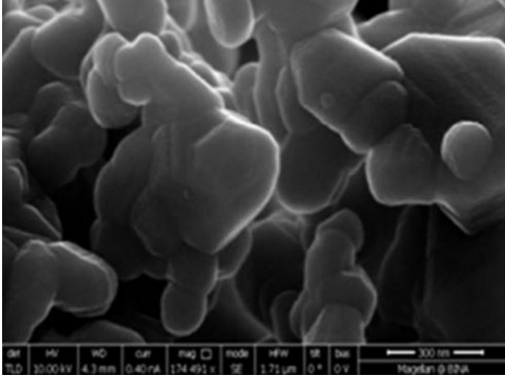
SEM – Strontium Dodecairon Nonadecaoxide Nanopowder
