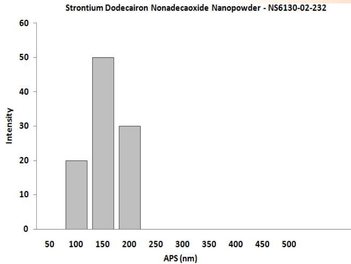
Particles Size Analysis - SrFe 12 O 19
