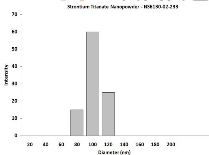
Size Analysis – SrTiO 3 Nanoparticles
