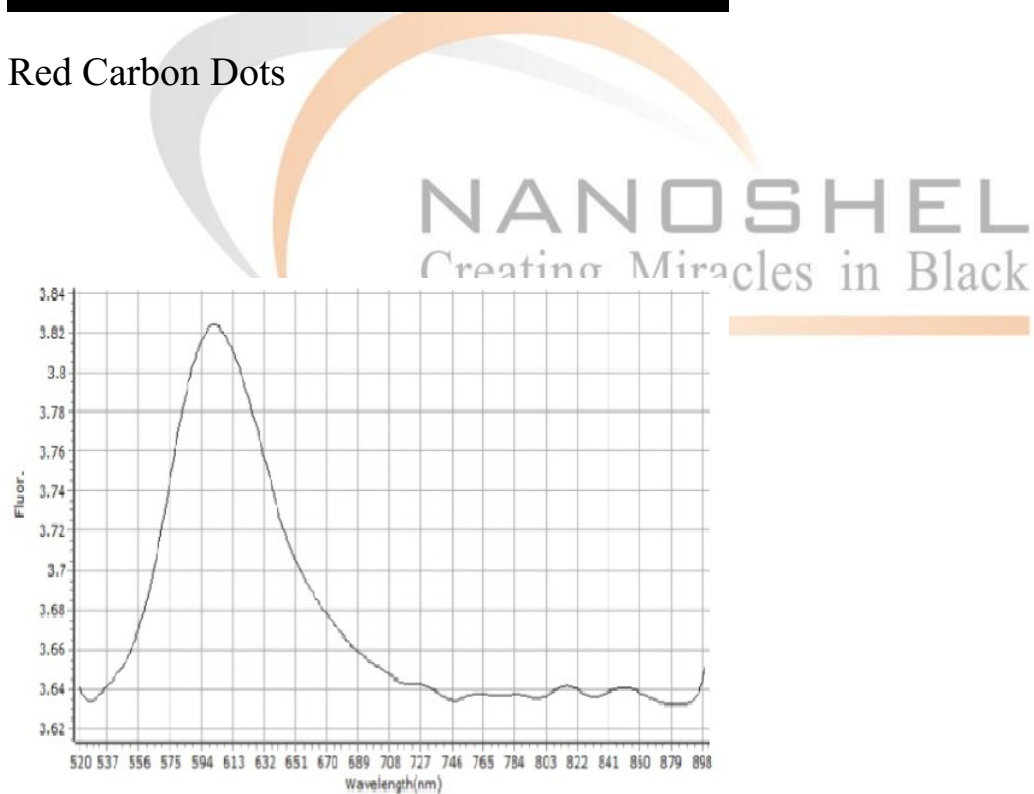
Fluorescence Spectroscopy - Red Carbon Dots
