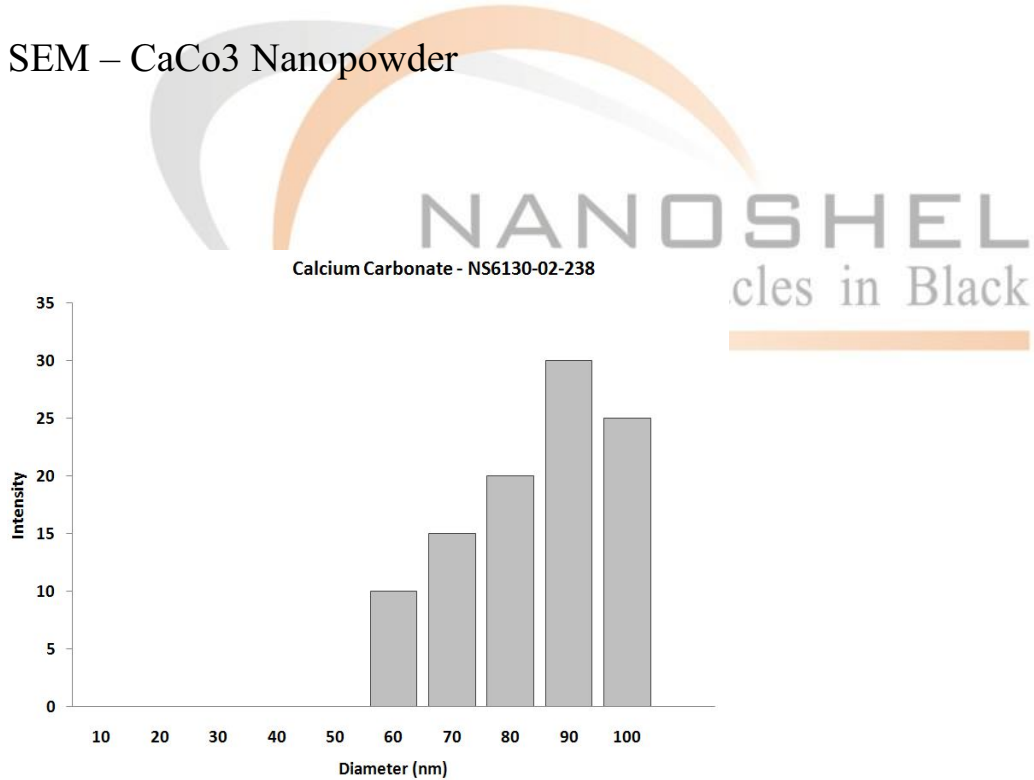
Calcium Carbonate Nanoparticles – Size Analysis
