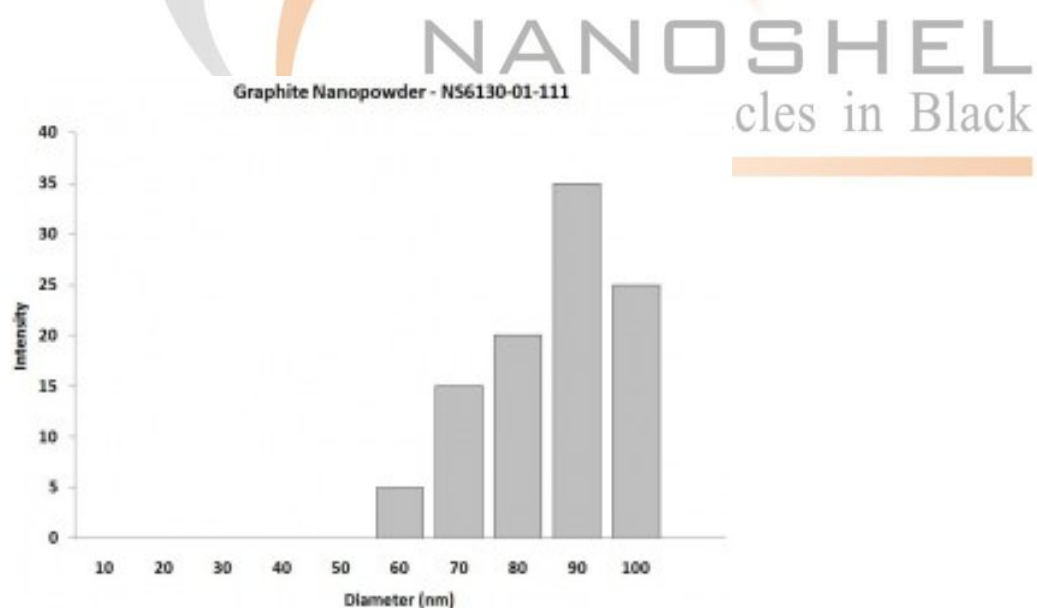
Particles Size Analysis - Graphite Nanoparticles
