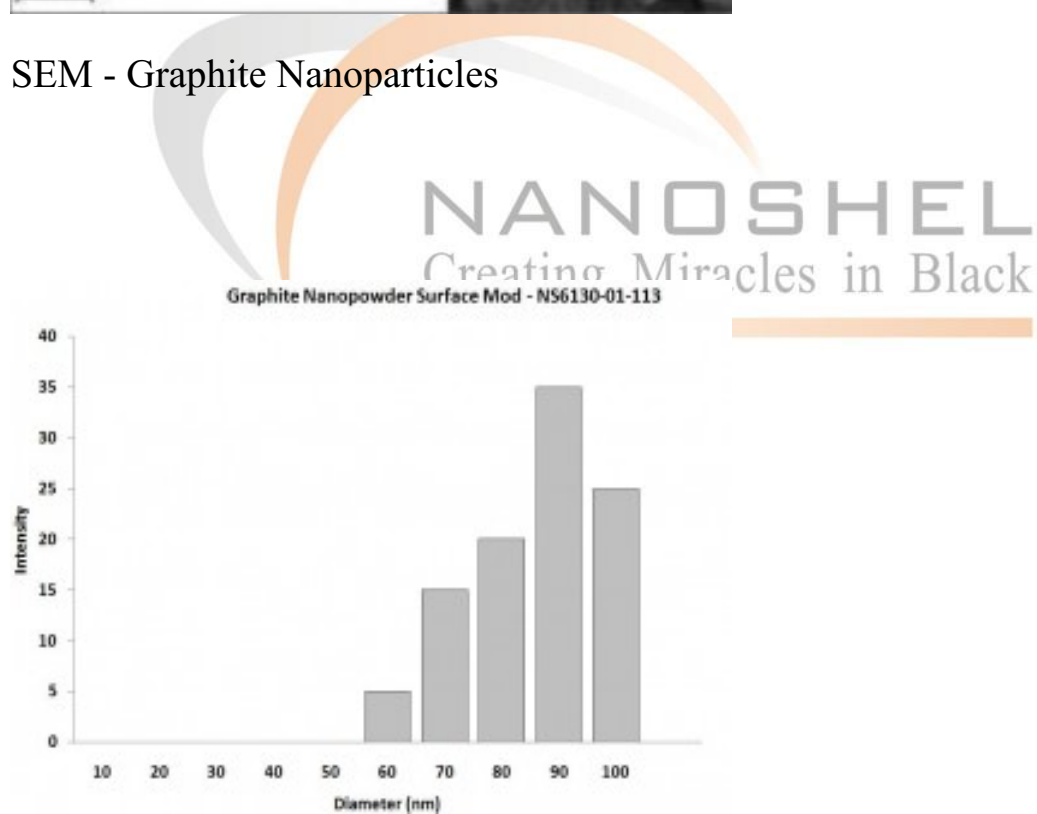
Particles Size Analysis - C Nanopowder
