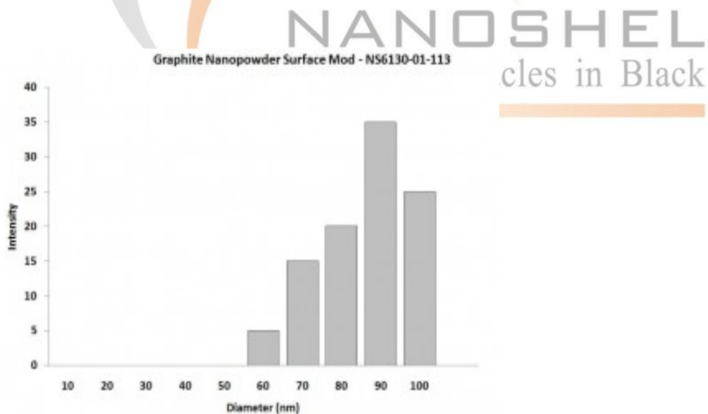
Particles Size Analysis - C Nanopowder
