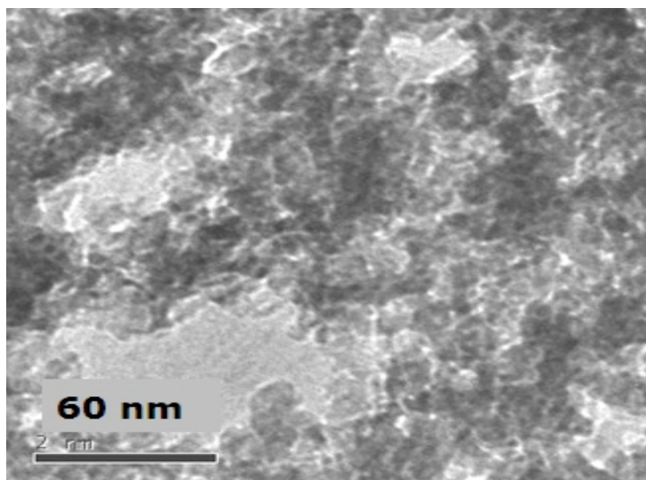
SEM – CdZnS Nanoparticles
