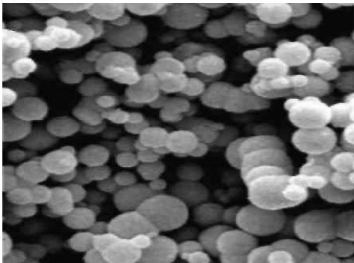
SEM - BaAl 2 O 4 Nanoparticles
