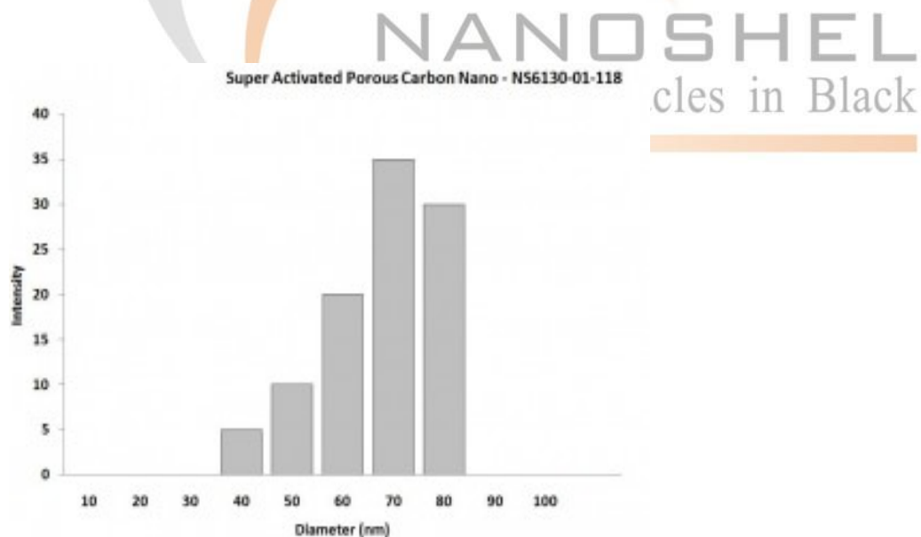
Particles Size Analysis - Charcoal Nanopowder
