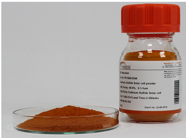
Cadmium Sulfide
