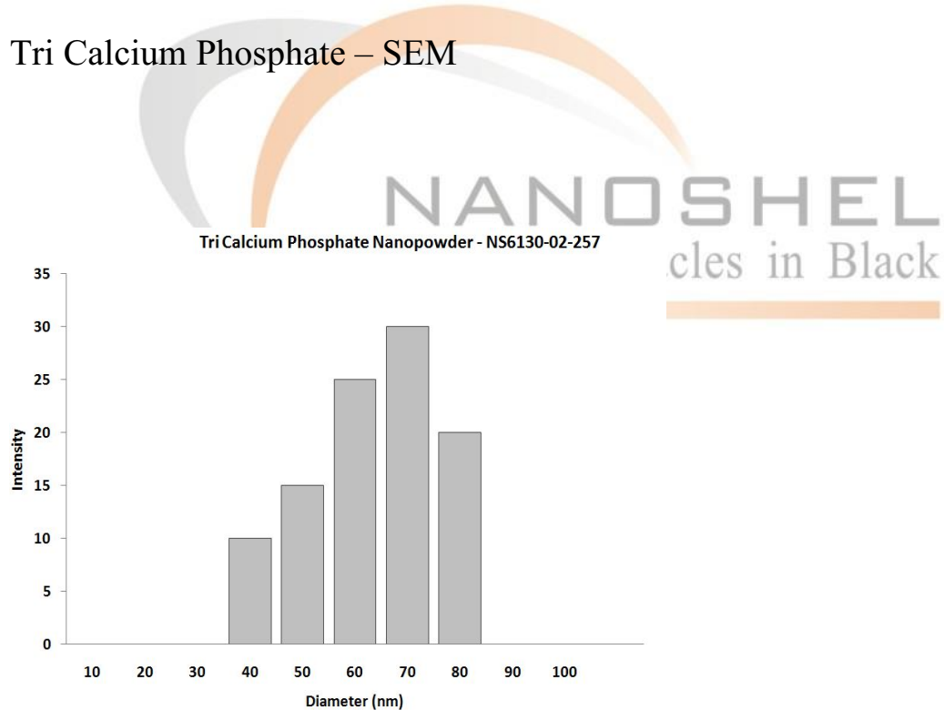
Tricalcium Phosphate Nanoparticles – Size Analysis
