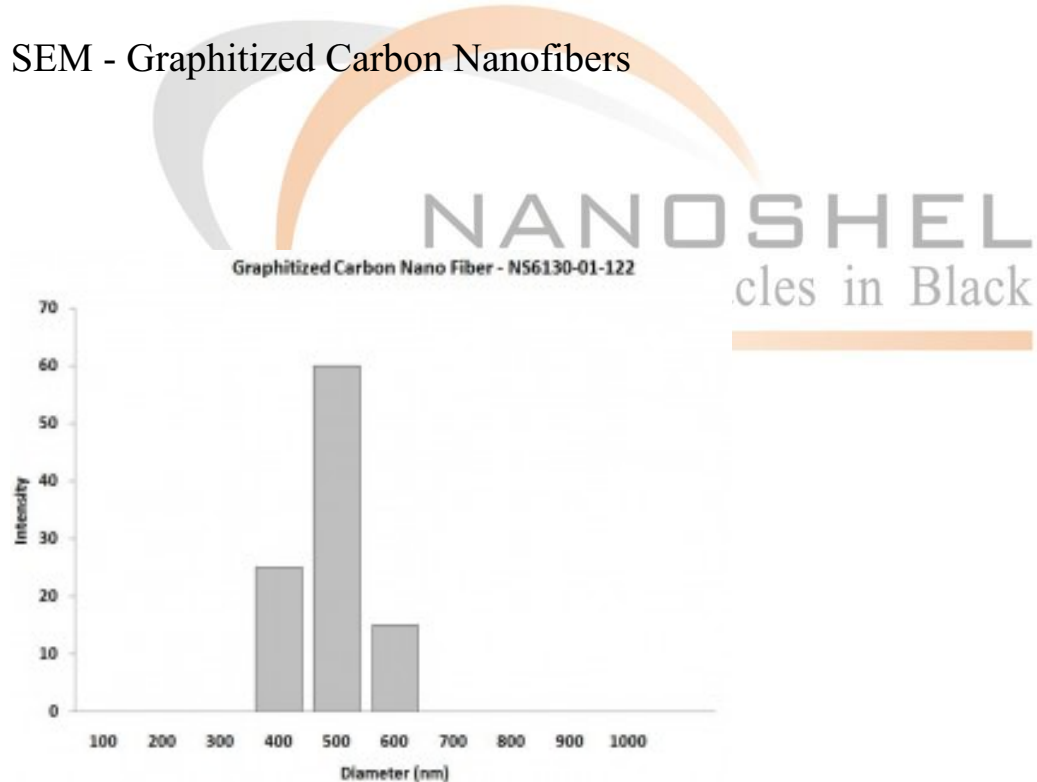
Size Analysis - Graphitized Carbon Nanofibers
