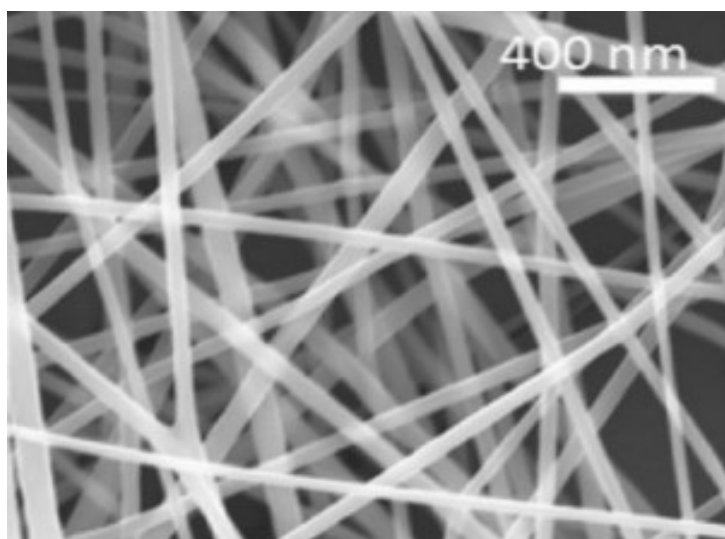
SEM - Graphitized Carbon Nanofibers
