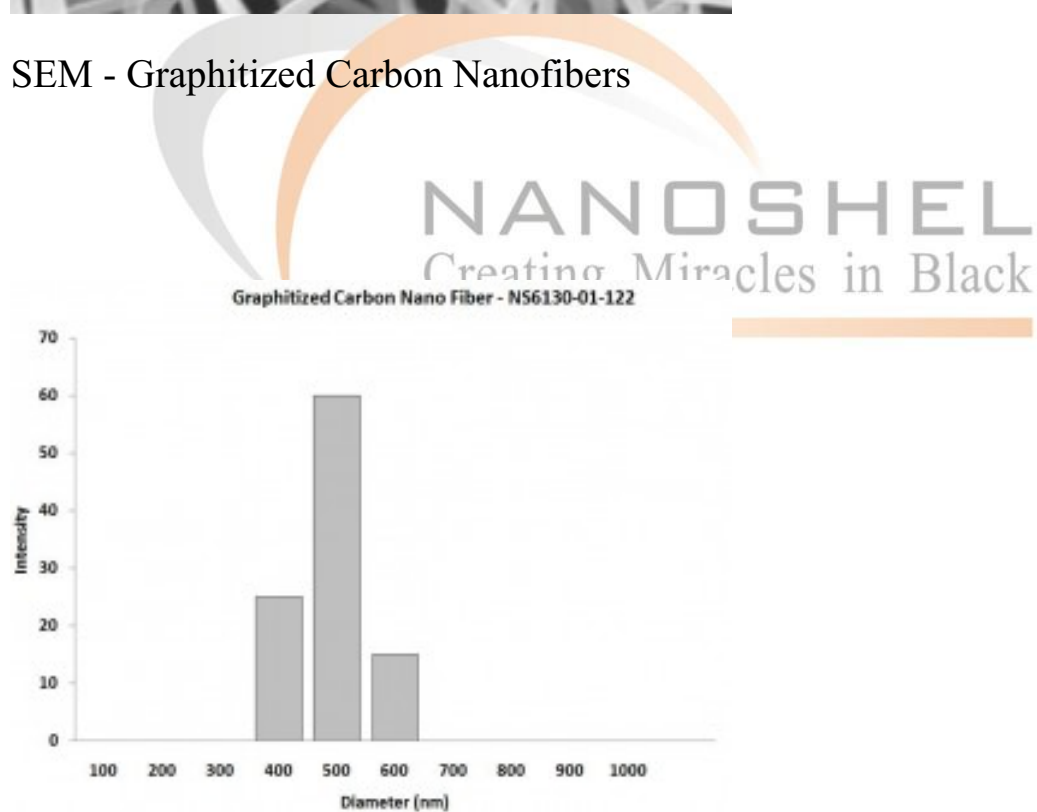
Size Analysis - Graphitized Carbon Nanofibers
