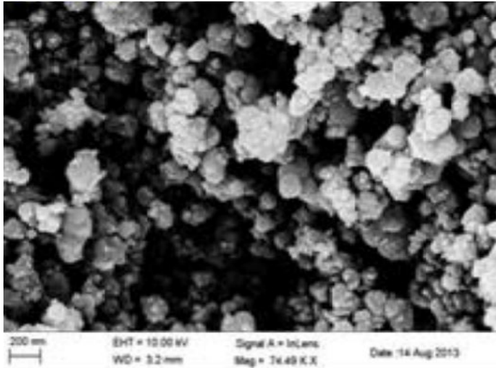
SEM – MnTiO 3 Nanoparticles
