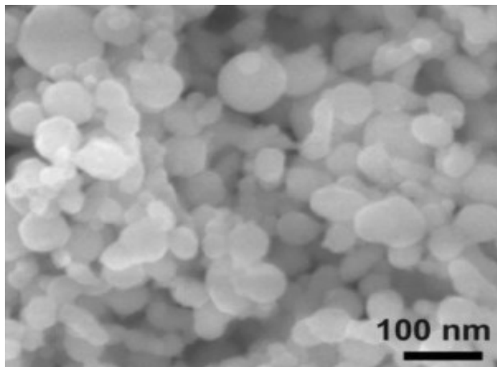
SEM - Cobalt Nanoparticles
