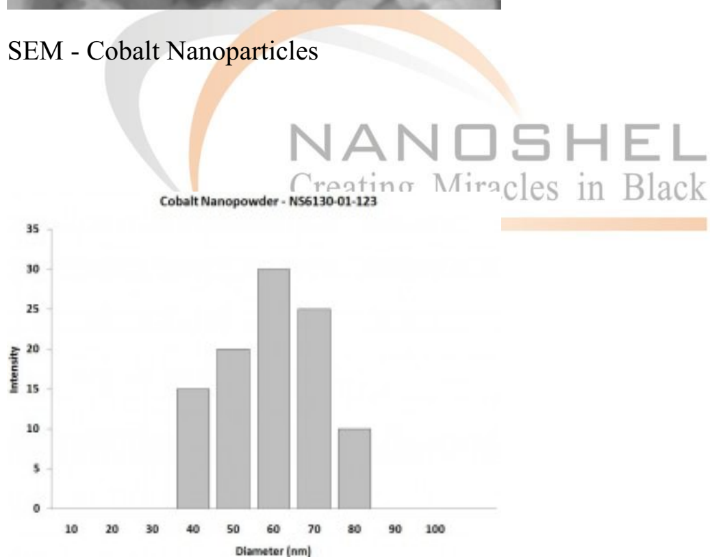
Particles Size Analysis - Co Nanopowder
