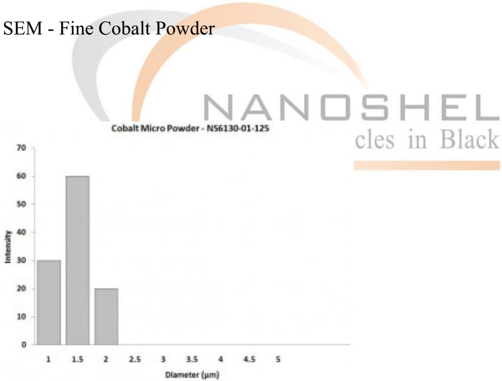
Particles Size Analysis - Co Powder
