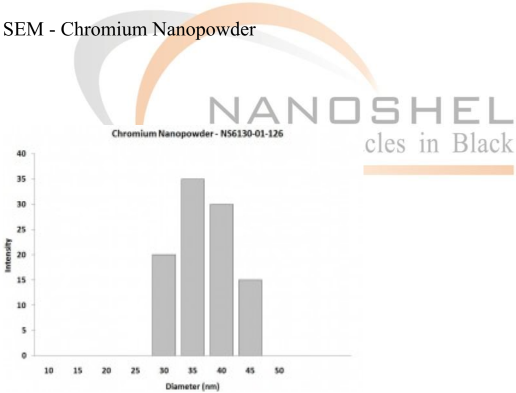
Particles Size Analysis - Cr Nanoparticles
