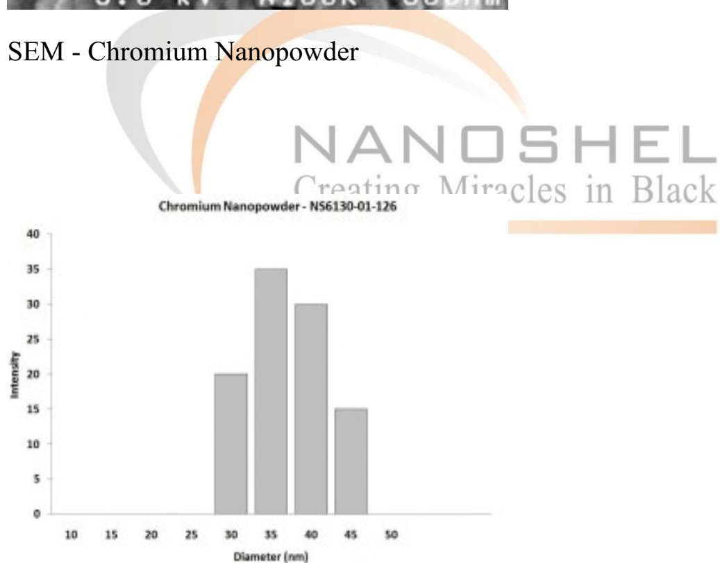
Particles Size Analysis - Cr Nanoparticles
