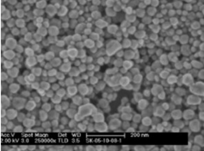
SEM - Copper Nanoparticle
