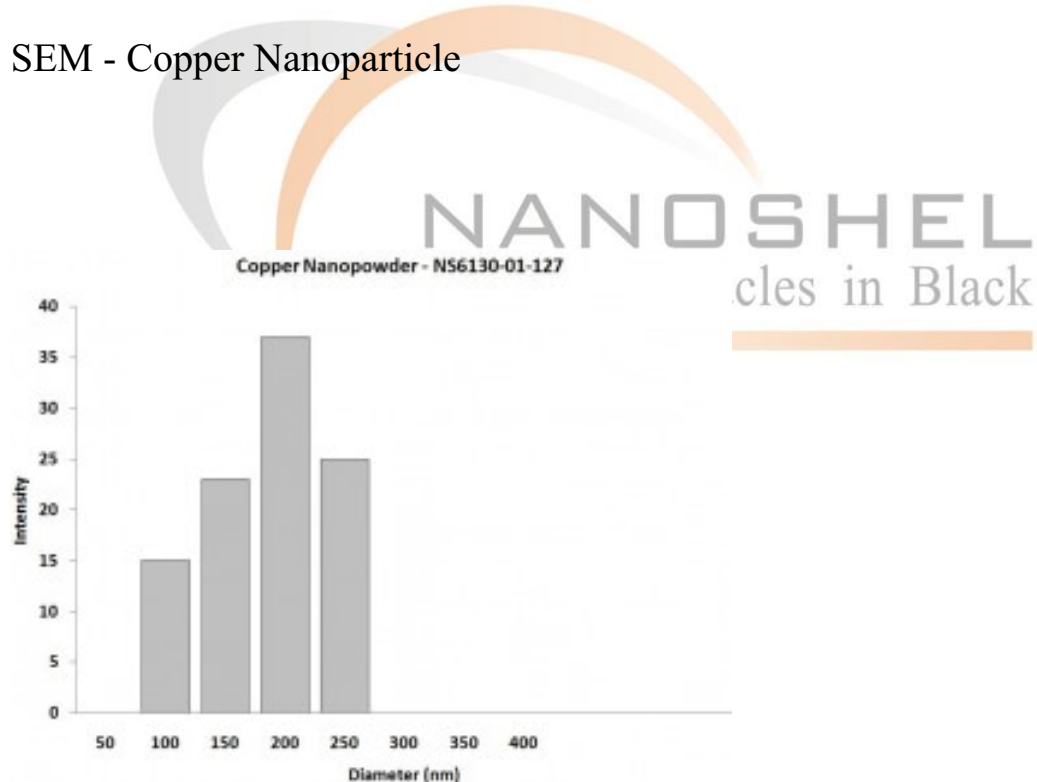
Particles Size Analysis - Cu Nanopowder
