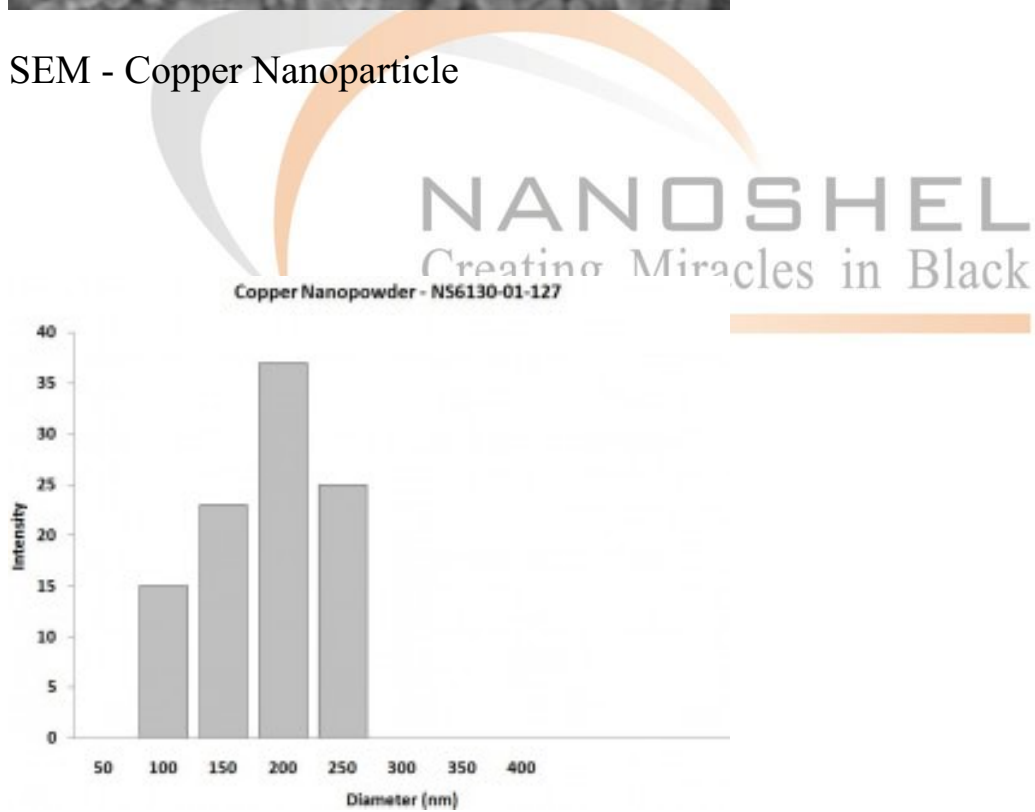
Particles Size Analysis - Cu Nanopowder
