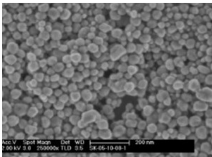
SEM - Copper Nanoparticle
